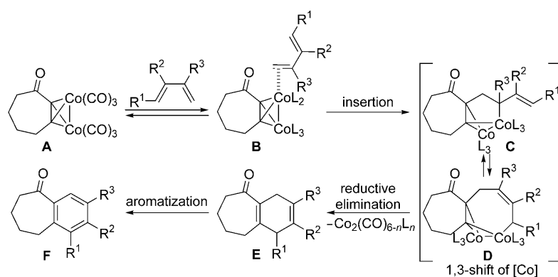
Scheme 1. Proposed reaction mechanism.
